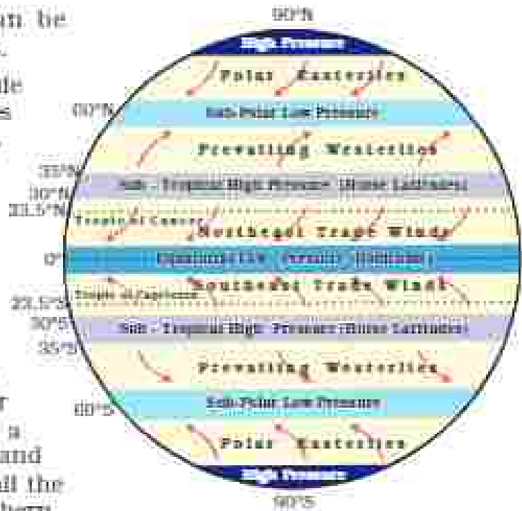
Fig. 4.4: Major Pressure Belts and Wind Systems
