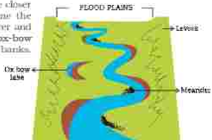
Fig. 3.5: Features made by a river at a flood plain.
